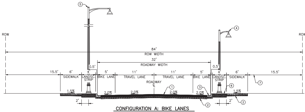
CONFIGURATION A: BIKE LANES
