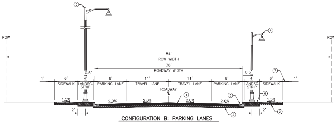
CONFIGURATION B: PARKING LANES
