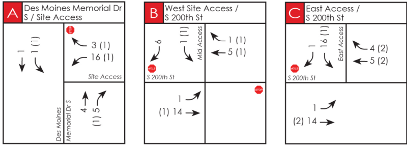
Figure 5: Weekday Peak Hour Project Trip Assignment (Site Driveways)
