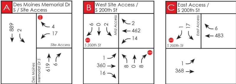
Figure 8: 2023 With Project Weekday Peak Hour Traffic Volumes (Site Driveways)
