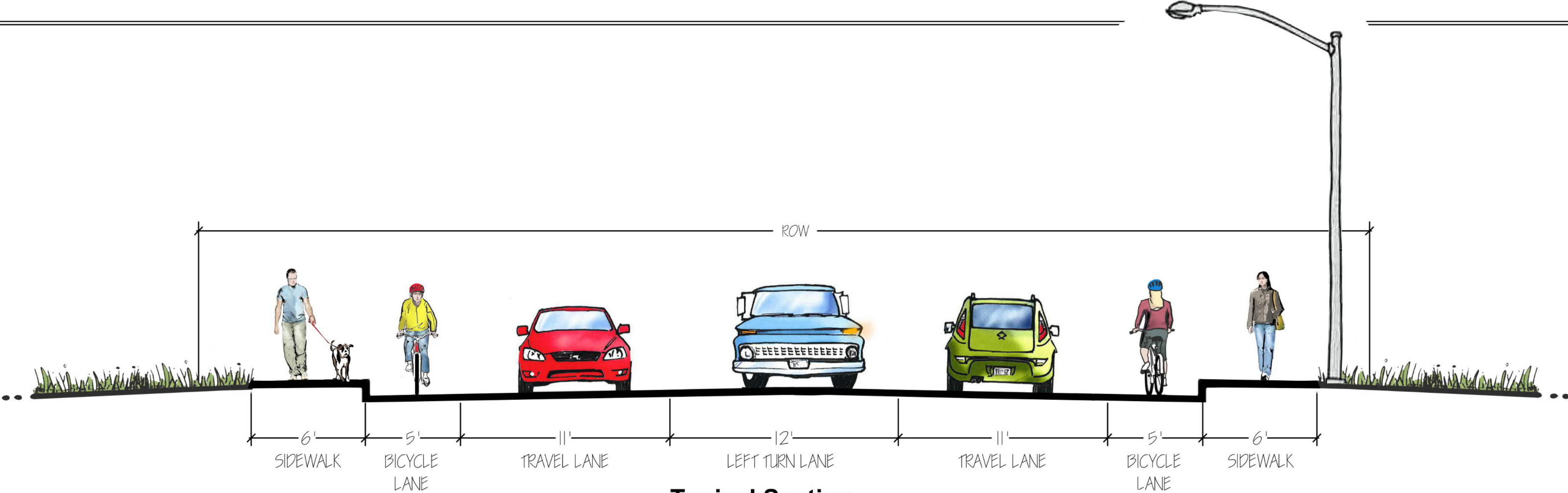
Typical Section Des Moines Memorial Drive
