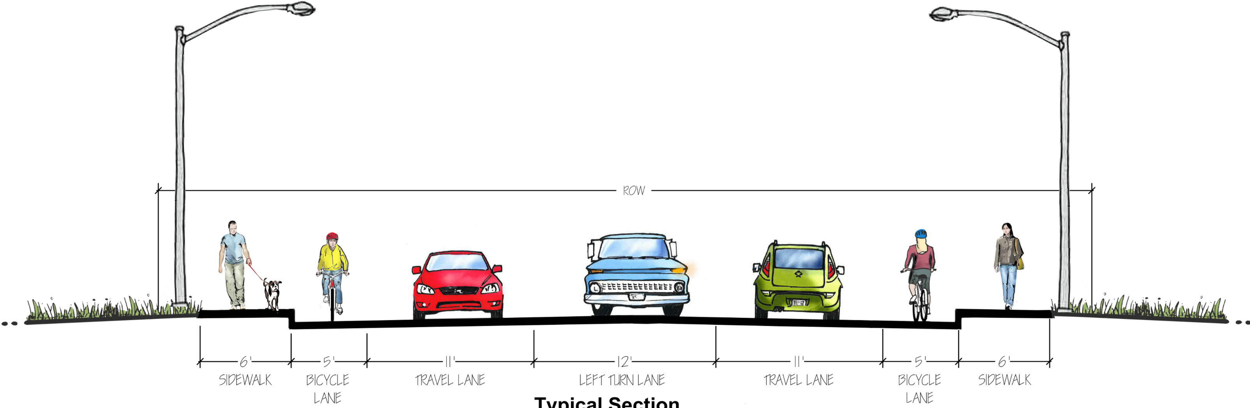
Typical Section South 200th Street - West Leg
