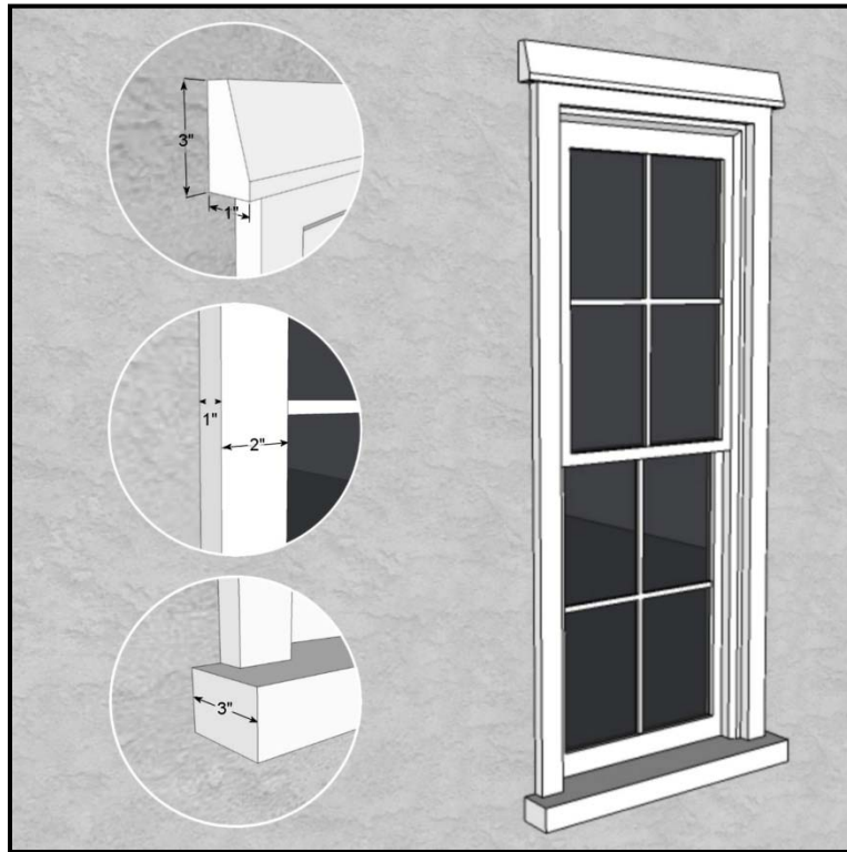
Figure 15.52539.320D Drip cap, sill, and trim details.
