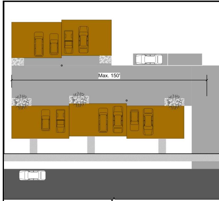
Figure 15.52539.240A Illustration of how the length of an auto court is measured.
