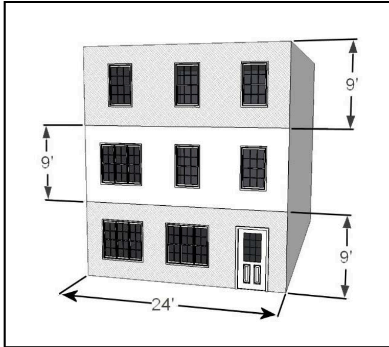
Figure 15.52539.320B Illustration of the window requirement. Each floor has a façade area of 216 square feet and requires 43.2 square feet of windows. The first floor has 66 square feet of windows, meeting the minimum requirement. The second floor has 46.5 square feet of windows, meeting the requirement. The third floor has 36 square feet of windows and DOES NOT meet the requirement.
