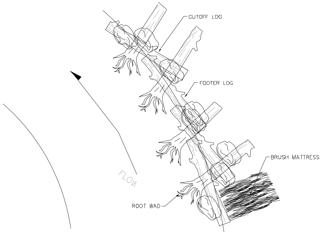
TYPICAL PLAN VIEW – NATURAL MATERIAL REVETMENT
