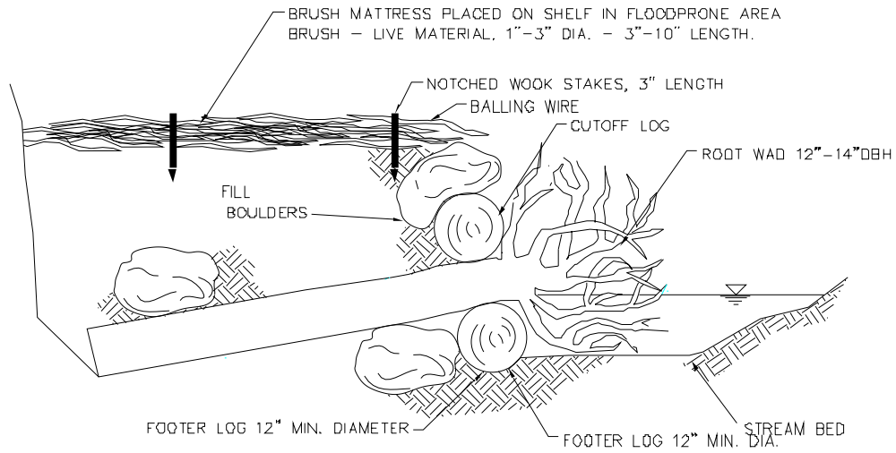
TYPICAL CROSS SECTION – NATURAL MATERIAL REVETMENT
